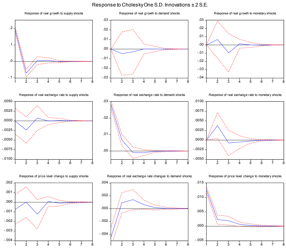
Figure 4.1: Impulse response for Gambia
