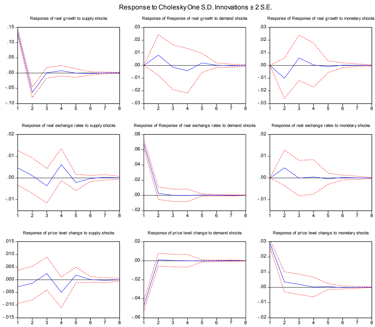
Figure 4.3: Impulse response for Guinea
